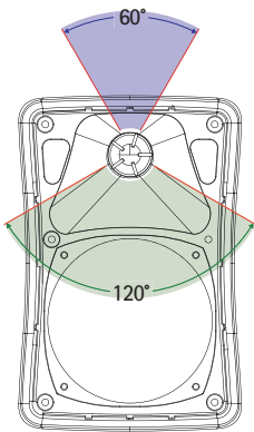
Horizontal Coverage
