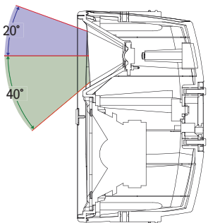
Vertical Coverage
