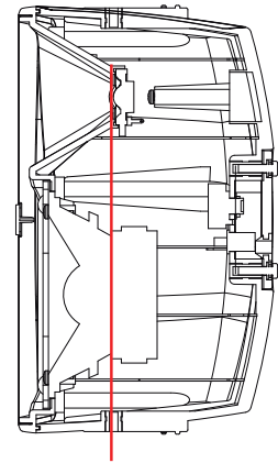
Physical Time Alignment Design
